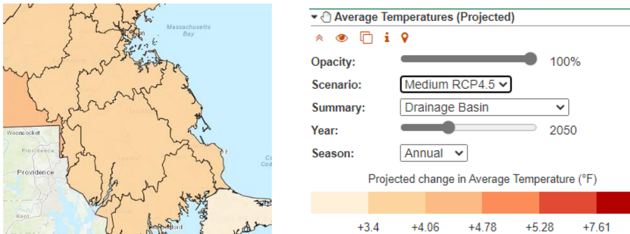
Figure 55: Average Temperature Projected 2050, Medium RCP 4.5
